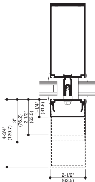
OPTIONAL COVERS
