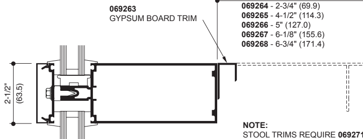
INTERIOR STOOL TRIM
