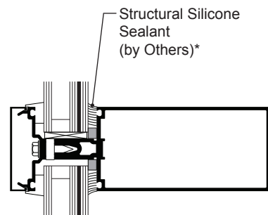
1-5/16" INFILL LARGE MISSILE (LMI)
