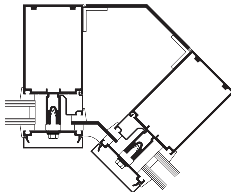
135° INSIDE CORNER
