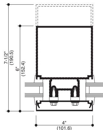
4" SIGHT LINE
