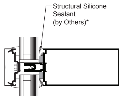
1-5/16" INFILL LARGE MISSILE (LMI) LEVEL E
