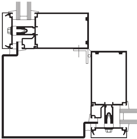
90° OUTSIDE CORNER
