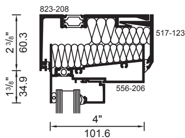
DEFLECTION HEAD (ALLOWS \pm 5/8 " (15.9) MOVEMENT)
