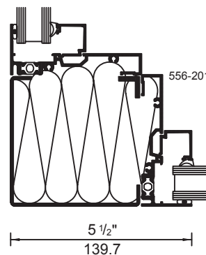
90° OUTSIDE CORNER
