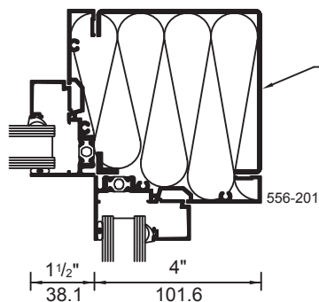
90° INSIDE CORNER
